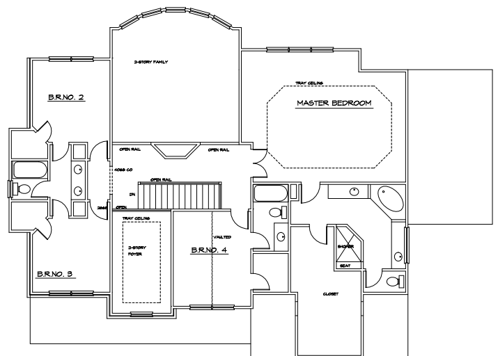
SECOND LEVEL
