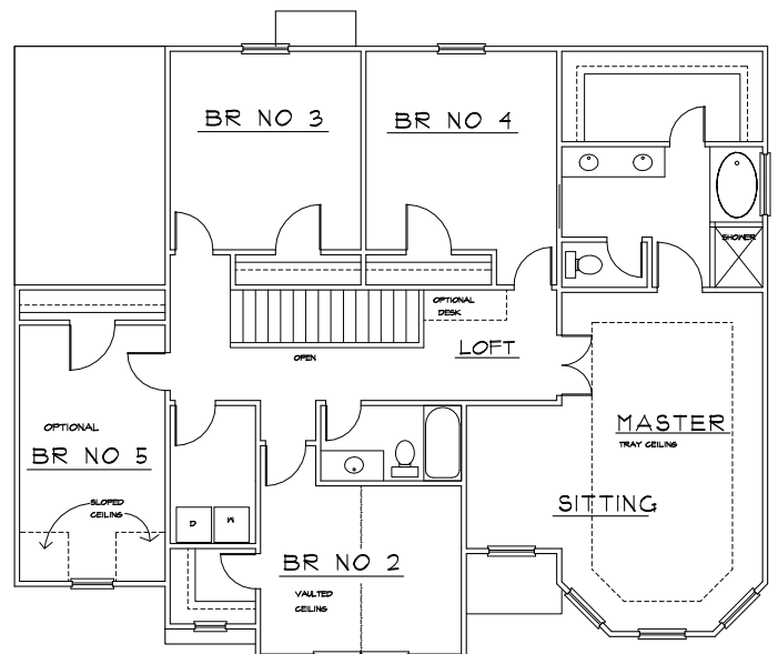
SECOND LEVEL
