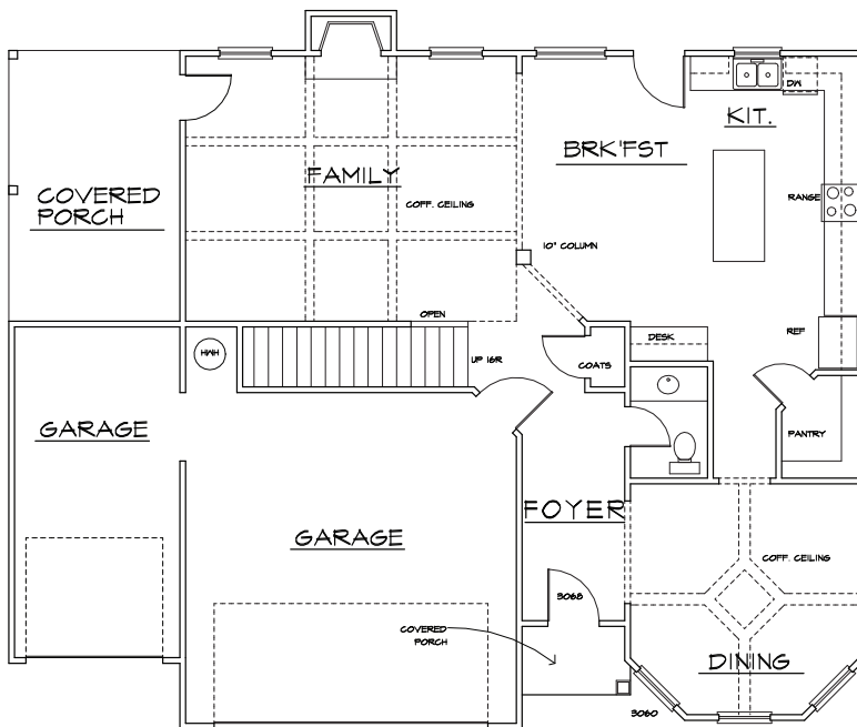
MAIN LEVEL
