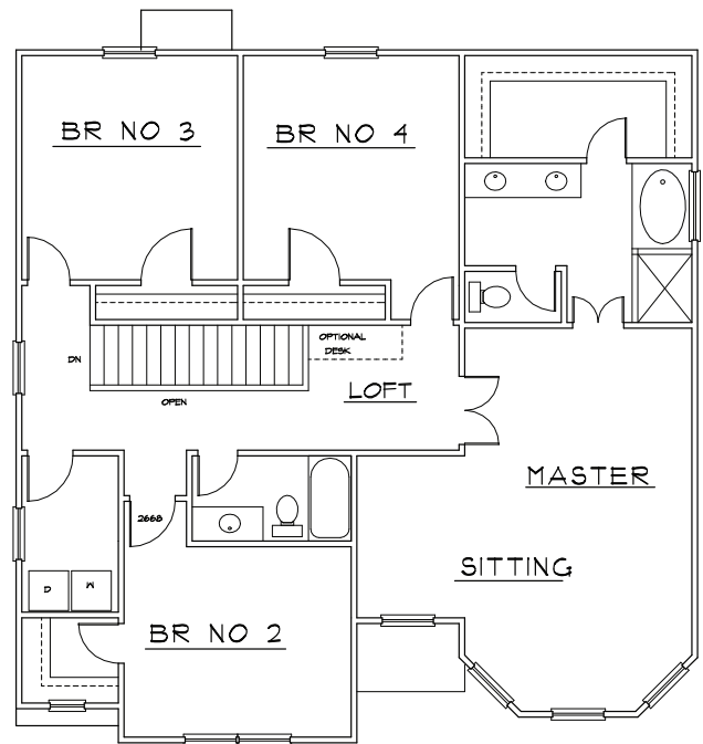
UPPER LEVEL
