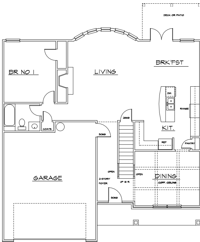
MAIN LEVEL
