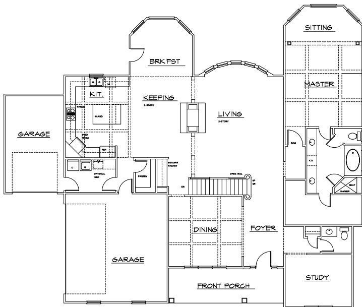
MAIN LEVEL
