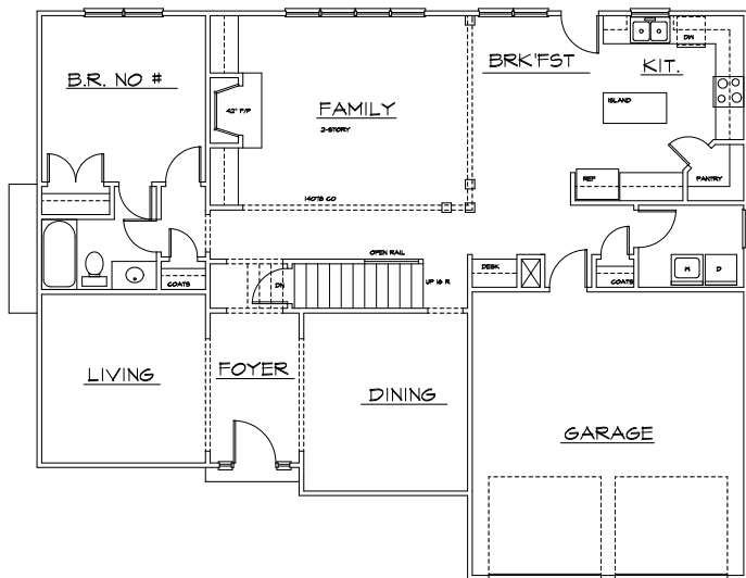
MAIN LEVEL
