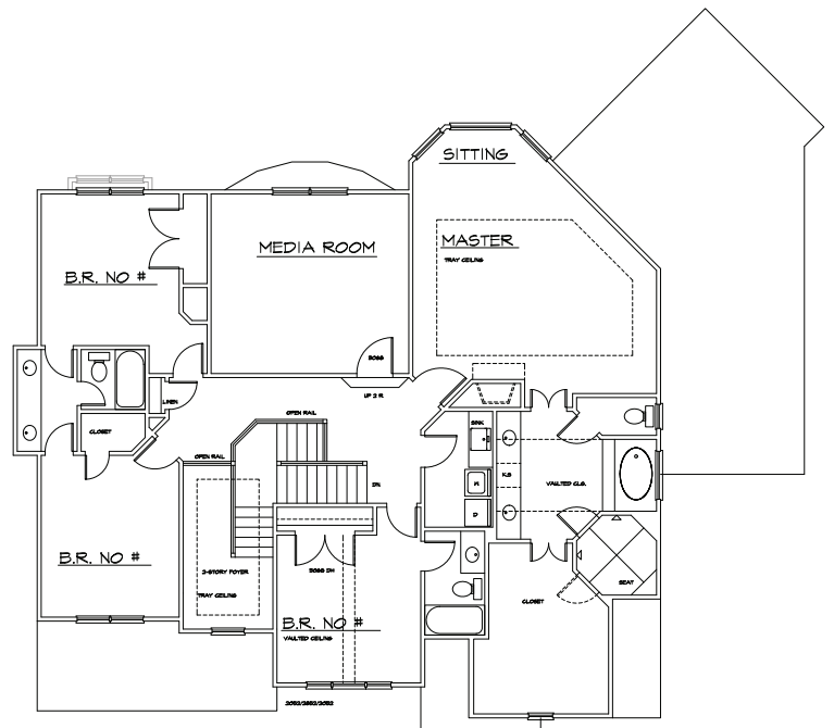
UPPER LEVEL
