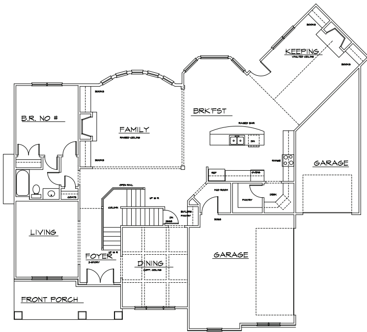
MAIN LEVEL
