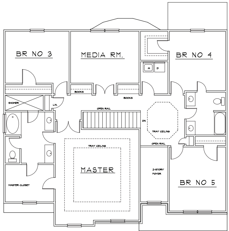
UPPER LEVEL
