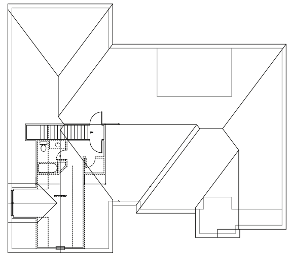
SECOND LEVEL
