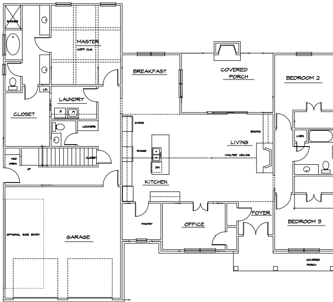
FIRST LEVEL
