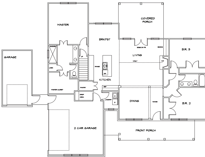
MAIN LEVEL
